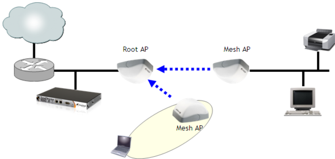
FIGURE 301 Mesh - wireless bridge topology
